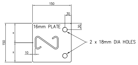
Z-POST ON BASE PLATE PLAN VIEW
